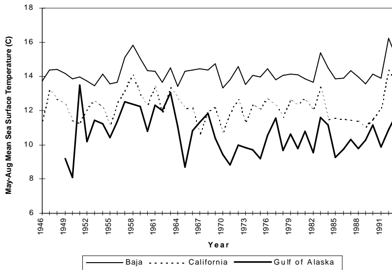
Figure 34. Average May-August sea surface temperatures at three near shore ocean sites.
