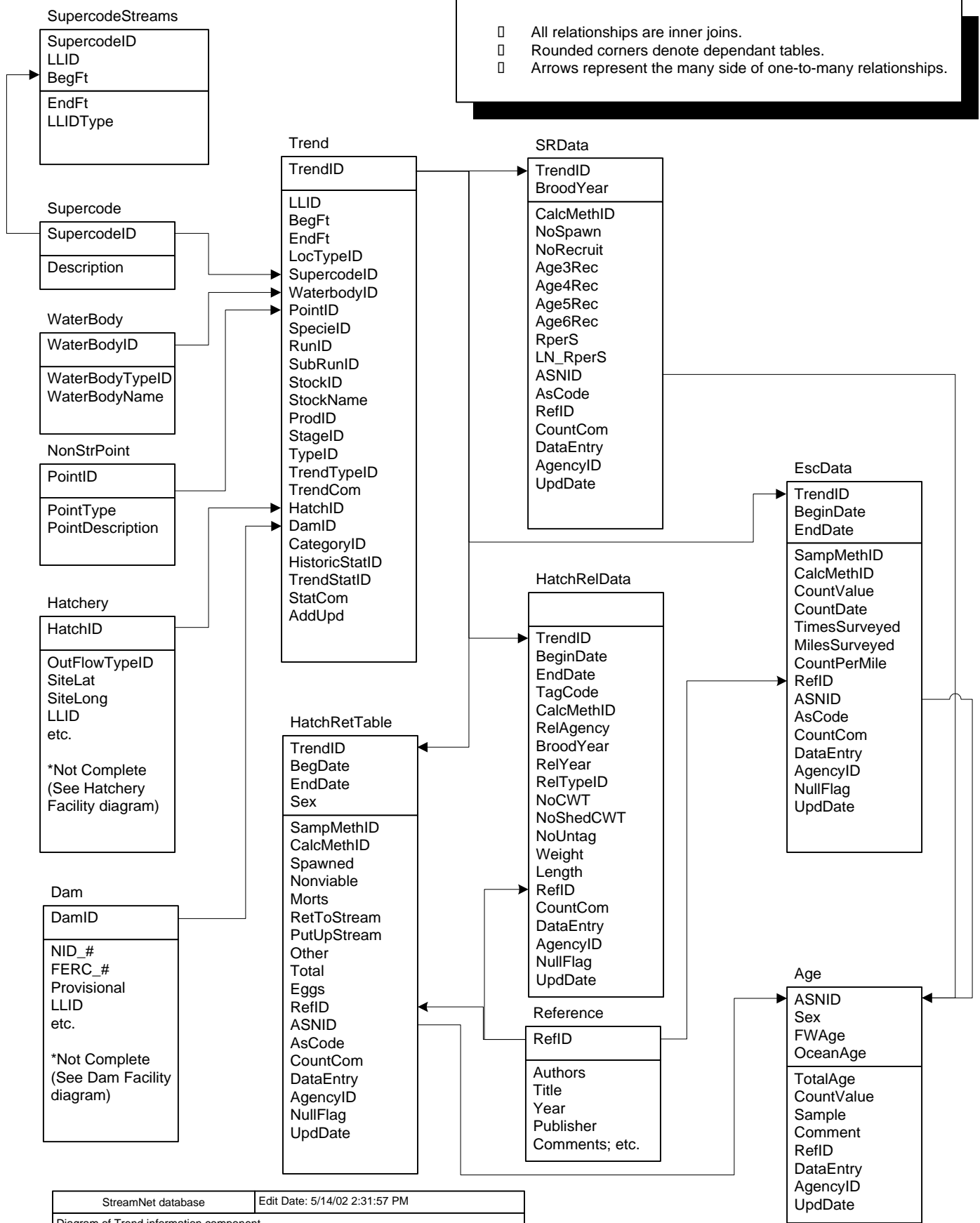
Figure 1. ER diagram for Trend (time series) data.
